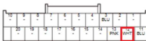
Wire side of female terminals
